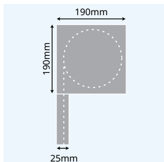
Headbox Zip Guide Extreme 190mm
