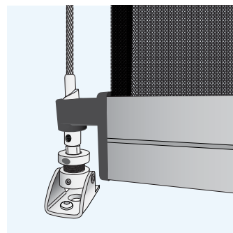
Wire Guide Ultra Lock
